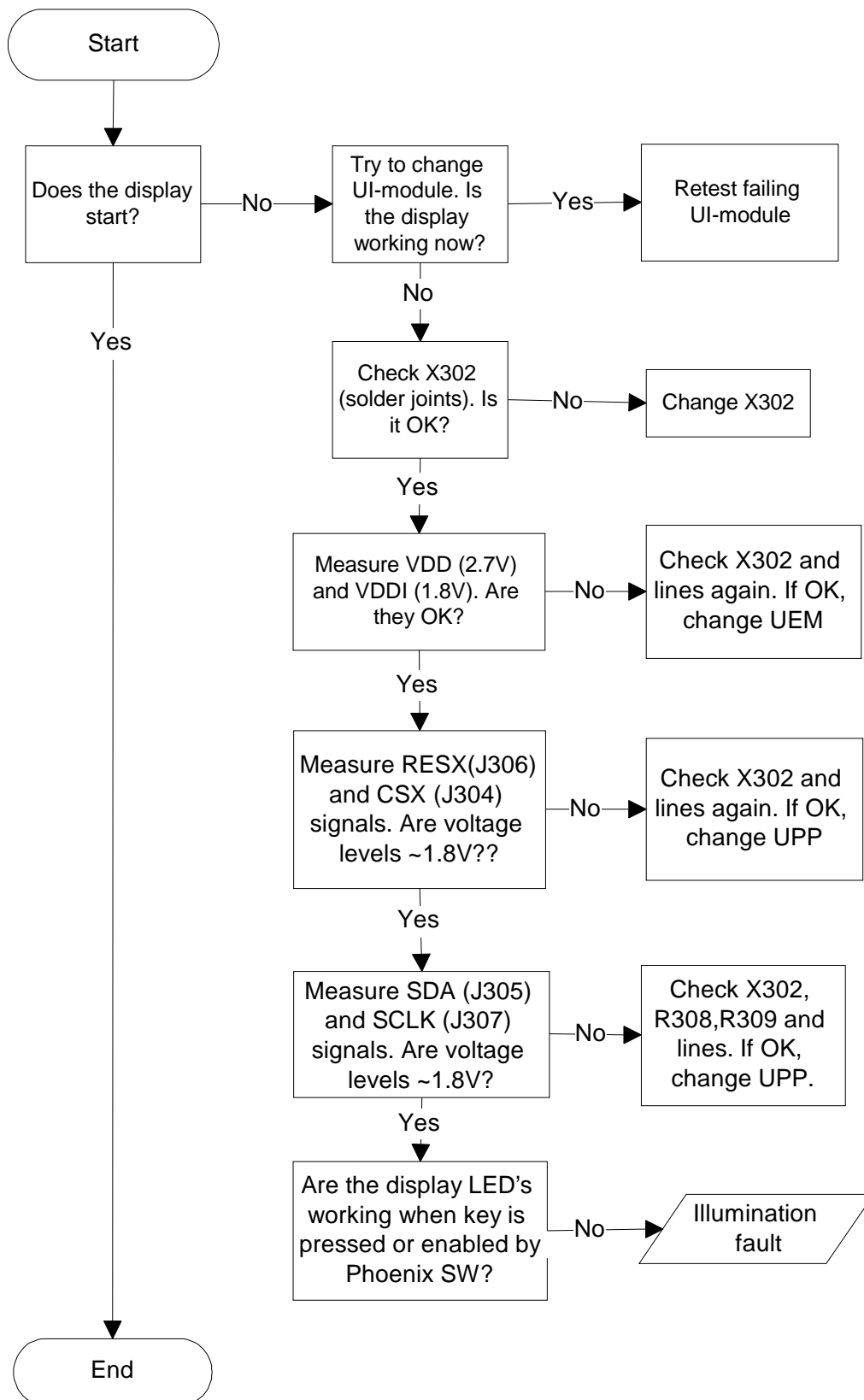
Figure 27: Display troubleshooting
