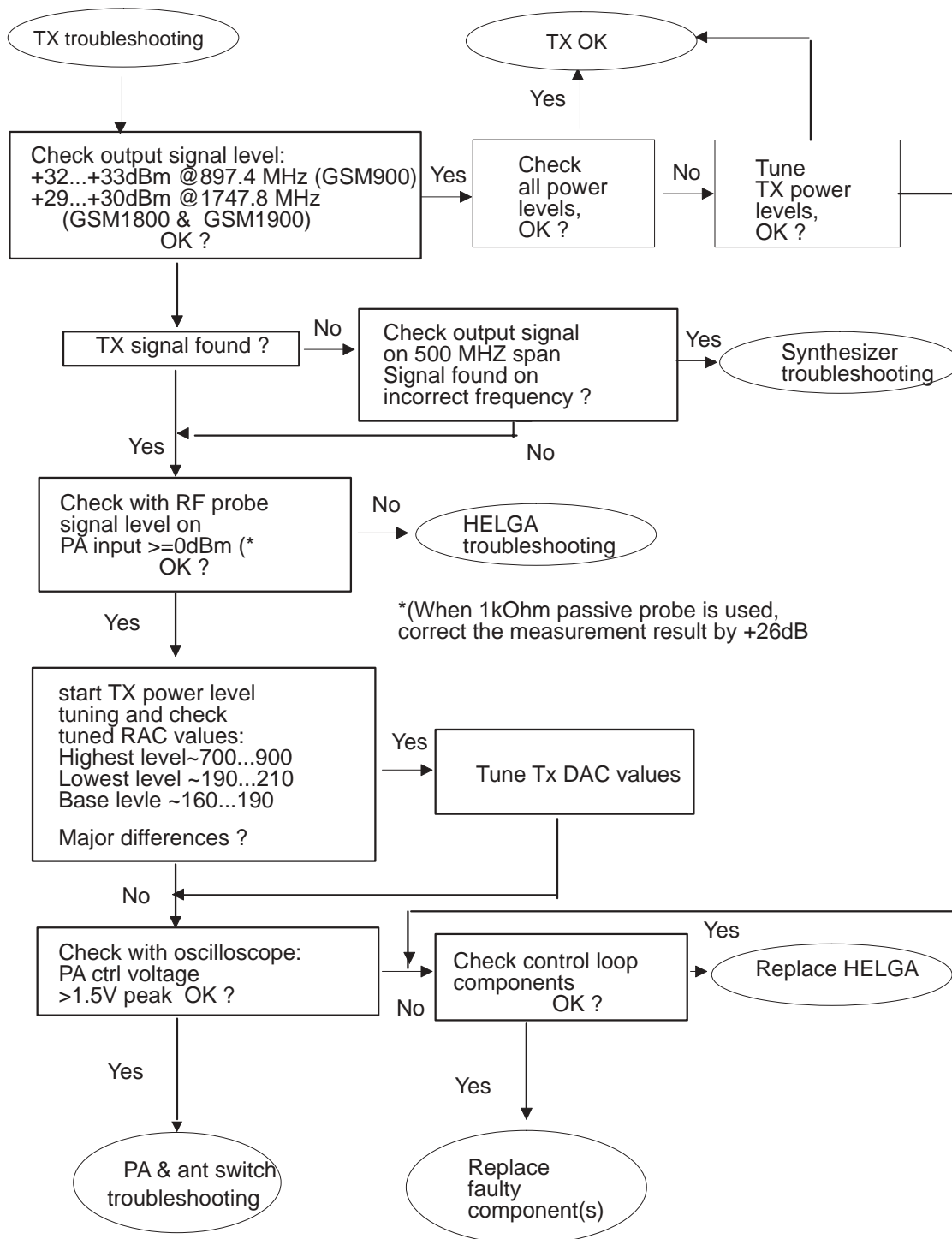
Figure 3: Transmitter troubleshooting
